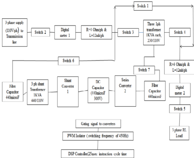
Figure 9: Detailed block diagram with specification for STATCOM
