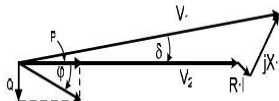
Figure2: Phasor diagram of transmission line model
