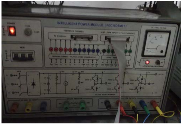
Figure 5: Intelligent Power Module
