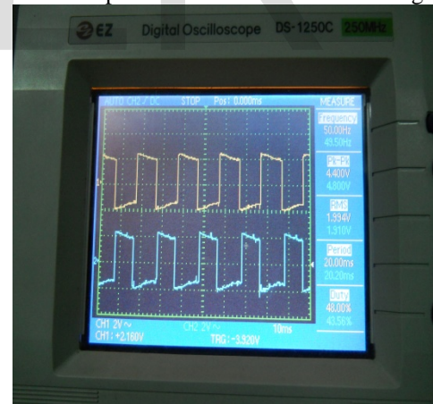
Figure 10: PWM pulse from DSP
