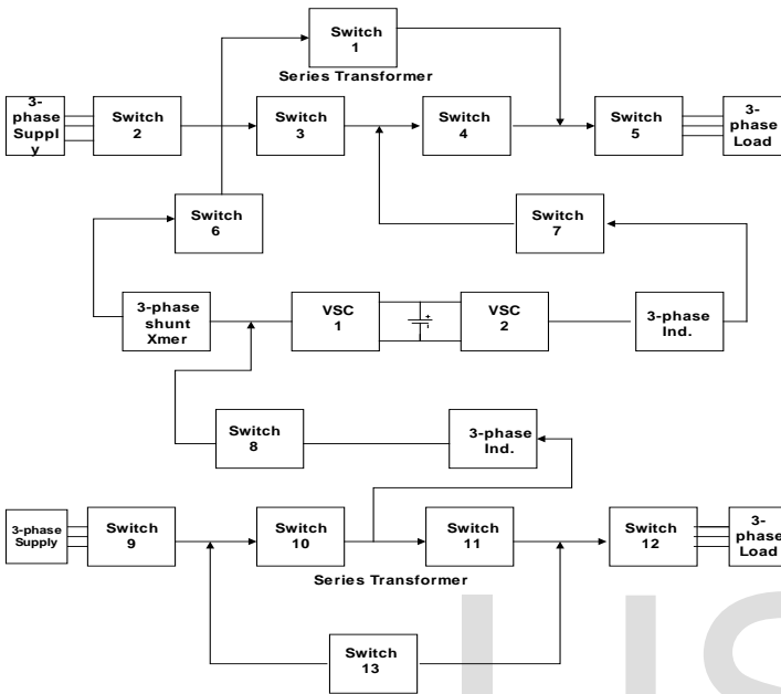
Figure 8: General block diagram
