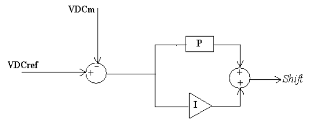
Figure 3: STATCOM DC voltage controller
